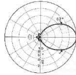
HORIZONTAL RADIATION PATTERN (at mid-band)
